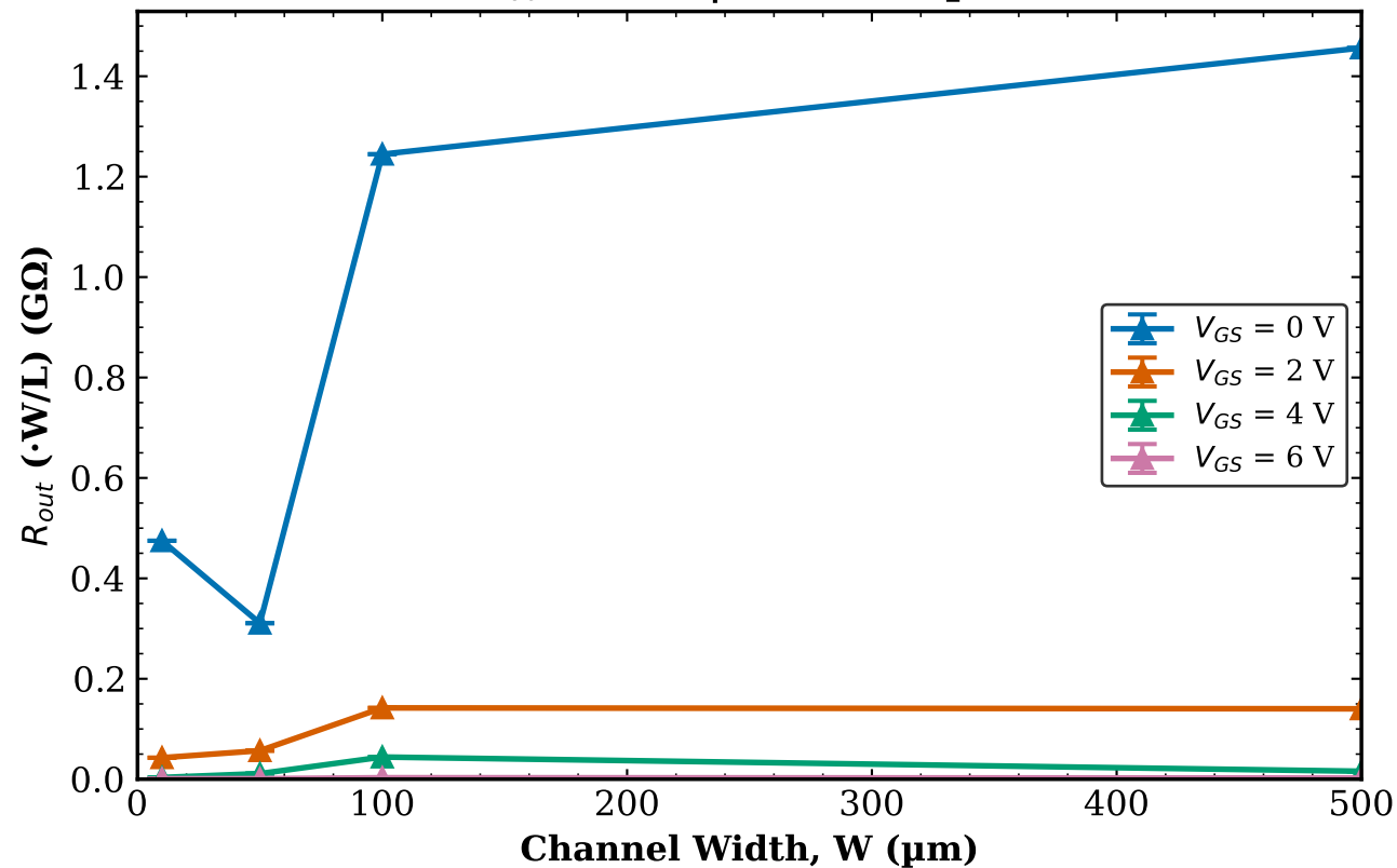
TFT2 Transistor 1 R_{out} vs W | L = 160\text{ }\mu\text{m}
